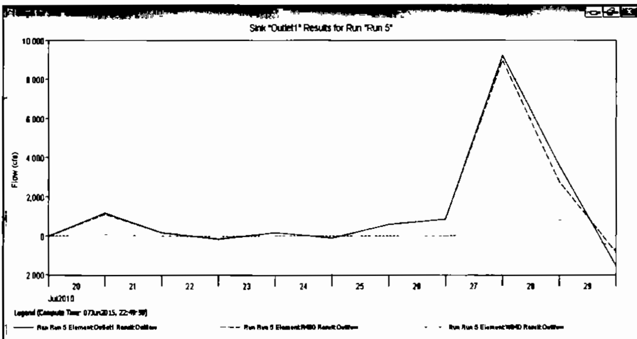
Fig 3 14: Graph for sink showing the difference between the outflow of hydrologic elements i.e. Outlet, Reach (R) and Subbasin (W).
