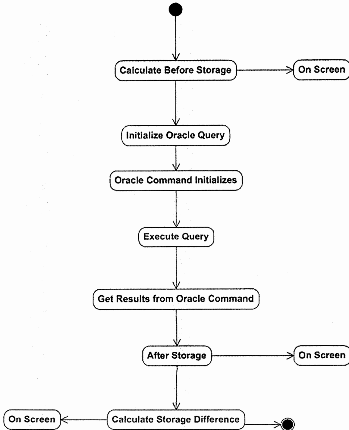
Fig 4-3 Detailed State Transition Diagram of Query Processing
