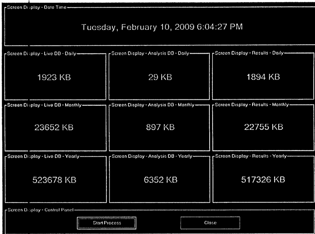
Fig 6-2 Result Screen
