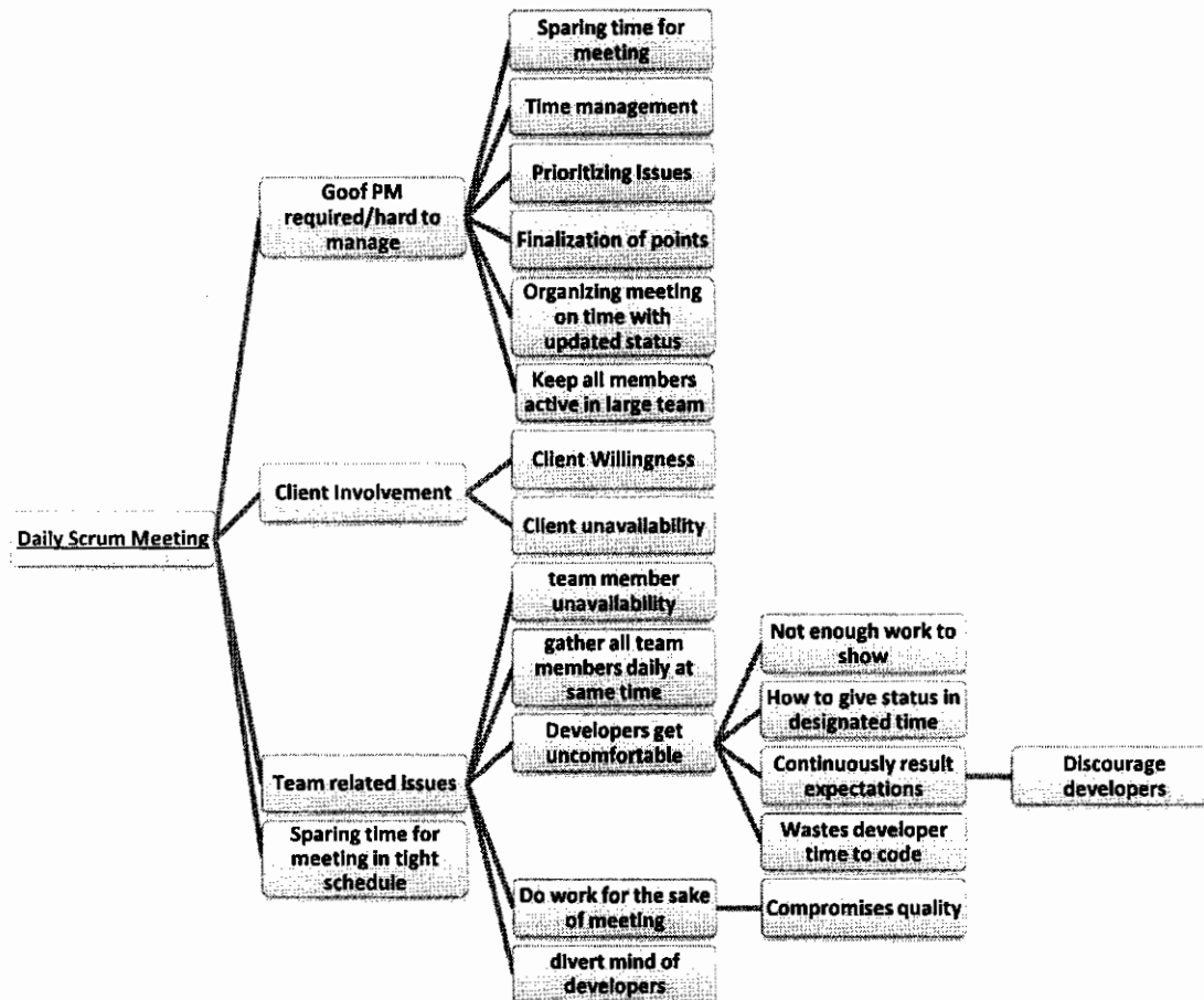
Figure 3.12: Challenges of Daily Scrum
