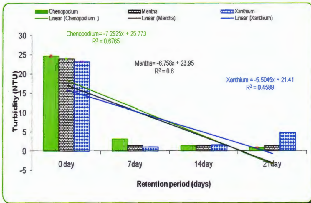
Figure 4.4. Effect of invasive plants on turbidity of the effluent
