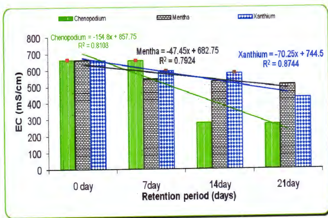
Figure 4.3. Effect of invasive plants on EC of the effluent
