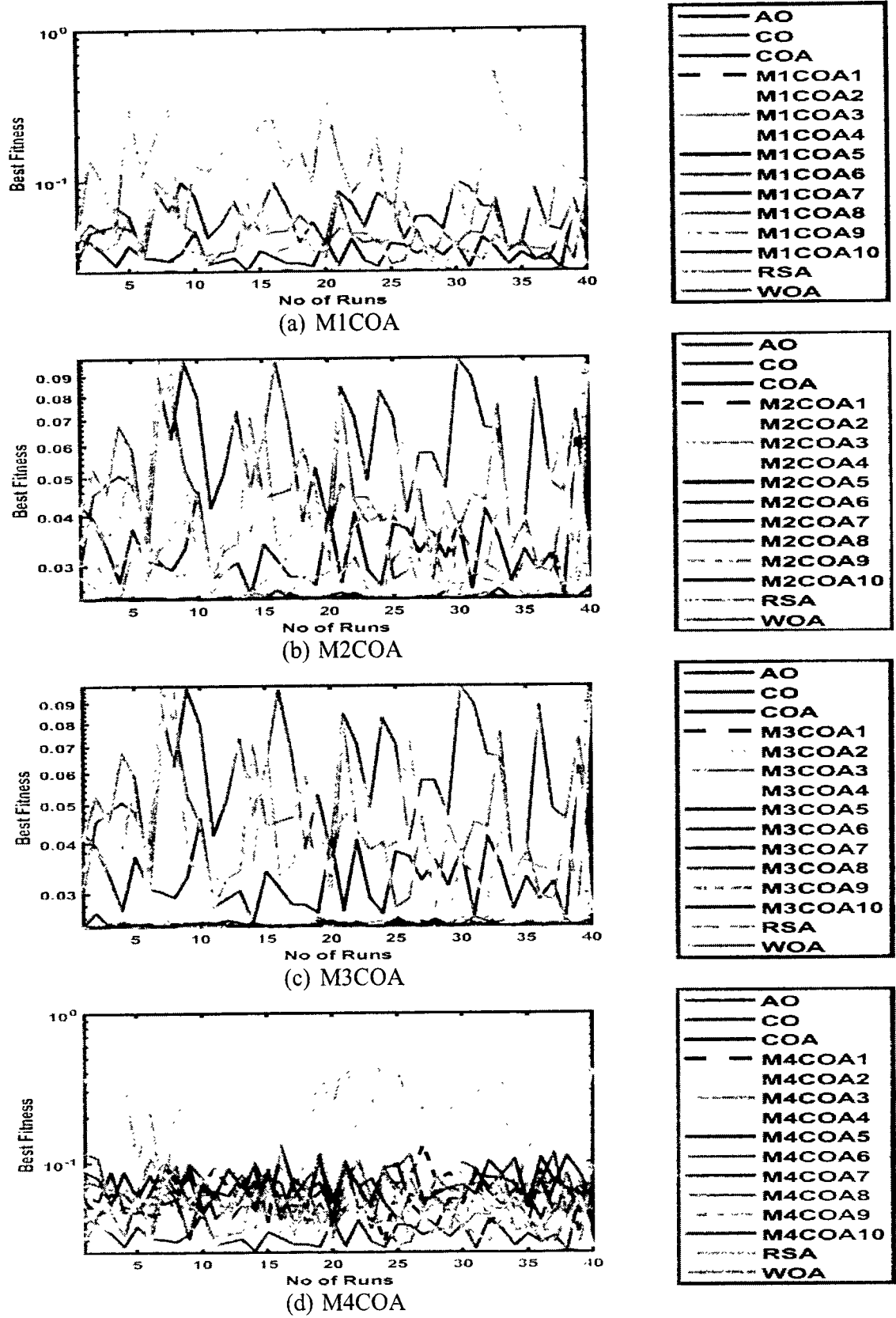
Figure 28: Statistical curves of M1COA1-M1COA10, M2COA1-M2COA10, M3COA1-M3COA10, M4COA1-M4COA10, CO, COA, WOA, and RSA at noise level m(k) = 1.9 \times 10^{-1}
