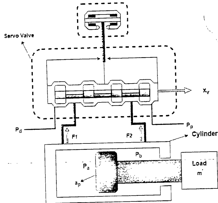
Figure 4: Electro-Hydraulic Actuator System
