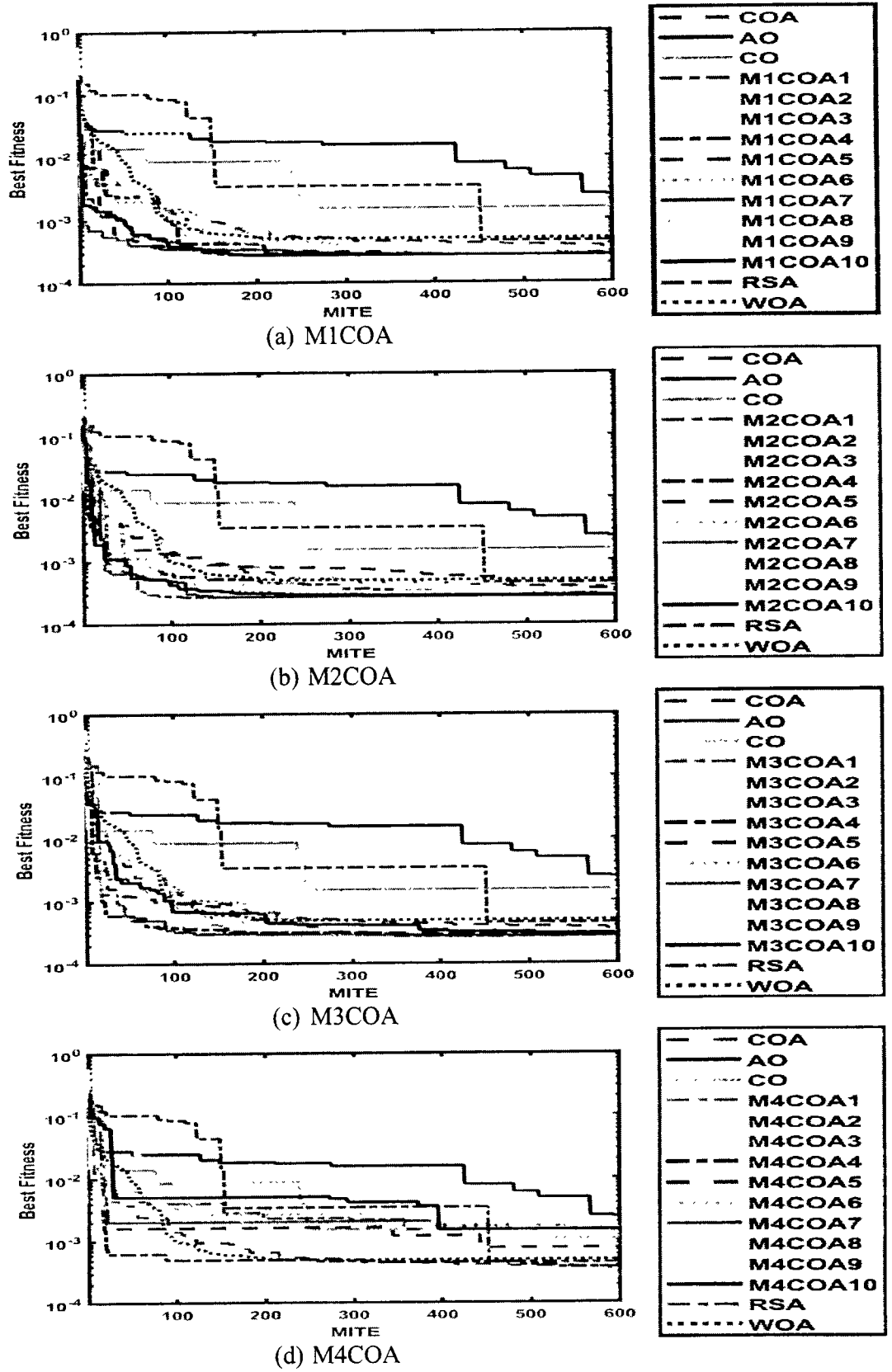
Figure 24: Convergence curves of M1COA1-M1COA10, M2COA1-M2COA10, M3COA1-M3COA10, M4COA1-M4COA10, CO, COA, WOA, and RSA at noise level m(k) = 1.9 \times 10^{-2}
