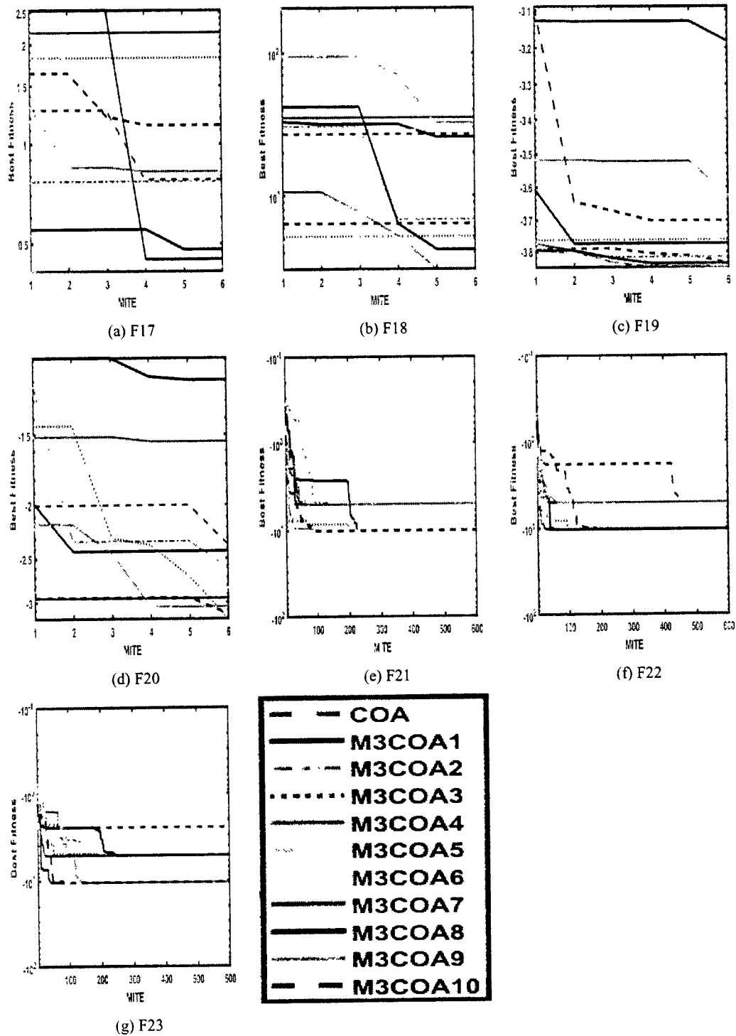
Figure 14: Analysis of F17-F23 for COA and M3COA1-M3COA10
